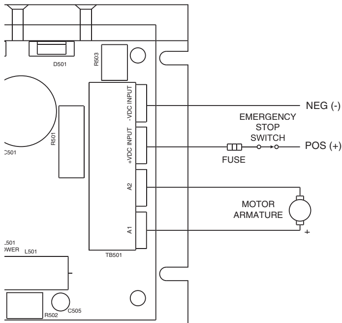
Figure 7. Power, Fuse and Motor Armature Connections
